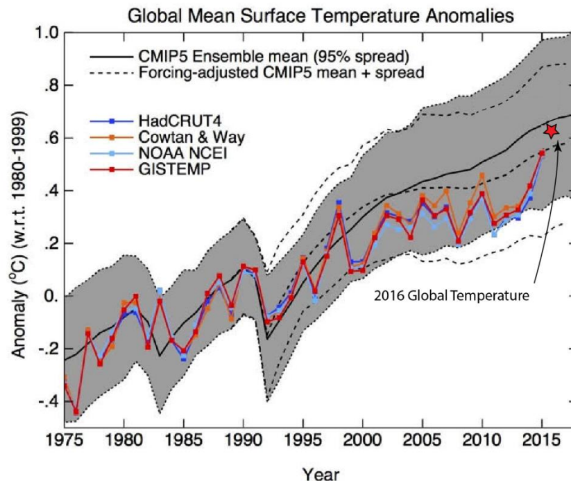
Figure 3. Comparison of Earth near-surface temperatures with climate models (Abraham, Cheng, Mann, in press).
